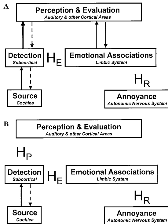
Figure 3 Classes of habituation. A , habituation of reactions, B , habituation of perception and reactions. Abbreviations: H R = habituation of reactions of the autonomic nervous system, H E = habituation of emotional reactions involving the limbic system, H P = habituation of perception.
