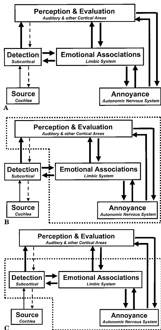
Figure 1 Block diagram outlining systems involved in clinically relevant tinnitus and changes occurring as a result of tinnitus habituation. Thickness of the arrows indicates the significance of a given connection. A , main diagram, B , upper loop, C , lower loop.
